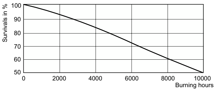
Life Expectancy Diagram - ML 250W E27 225-235V SG SLV/12
