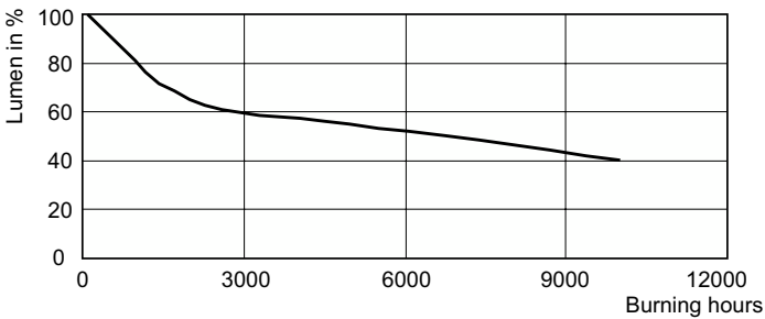
Lumen Maintenance Diagram - MASTERC CDM-R111 35W/942 GX8.5 10D 1CT/6
