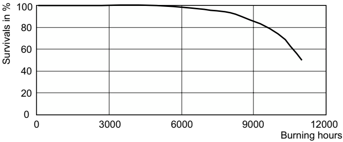
Life Expectancy Diagram - MASTERC CDM-R111 70W/942 GX8.5 10D 1CT/6
