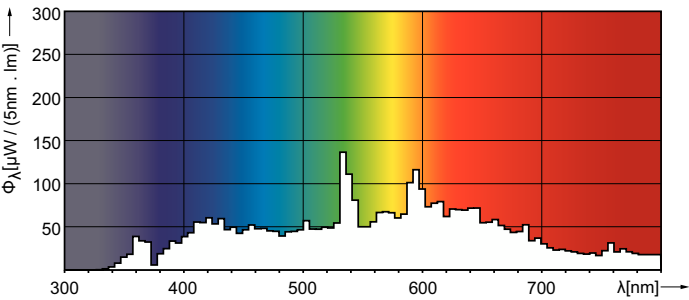
Spectral Power Distribution Colour - MASTERC CDM-R111 70W/942 GX8.5 10D 1CT/6
