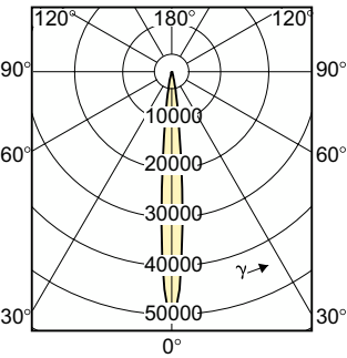
Light Distribution Diagram - MASTERC CDM-R111 70W/942 GX8.5 10D 1CT/6
