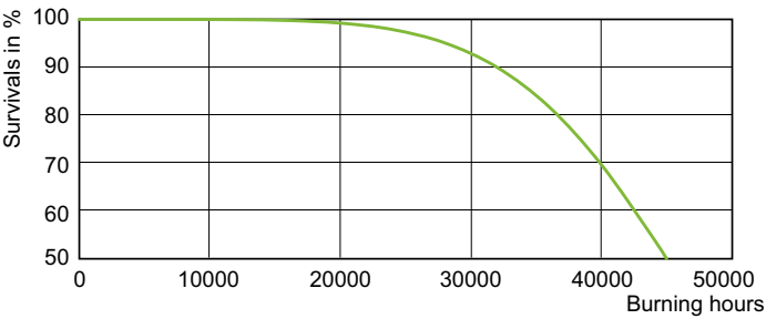
Life Expectancy Diagram - MST SON-T APIA Plus Xtra 400W HF E40
