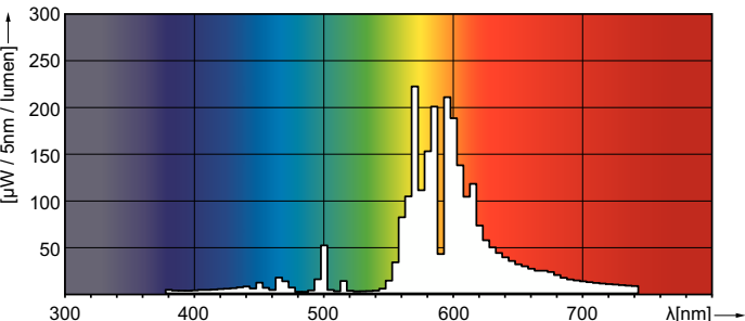
Spectral Power Distribution Colour - MST SON-T APIA Plus Xtra 400W HF E40
