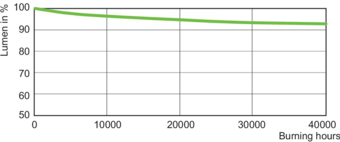
Lumen Maintenance Diagram - MST SON-T APIA Plus Xtra 400W HF E40
