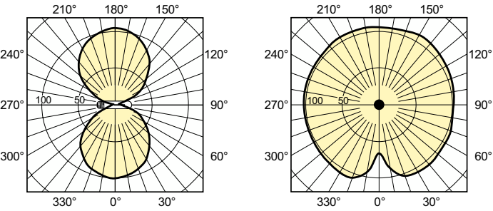
Light Distribution Diagram - MST SON-T APIA Plus Xtra 400W HF E40
