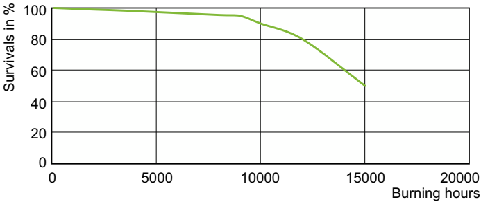
Life Expectancy Diagram - MC CDM-R Elite 50W/930 E27 PAR30L 30D
