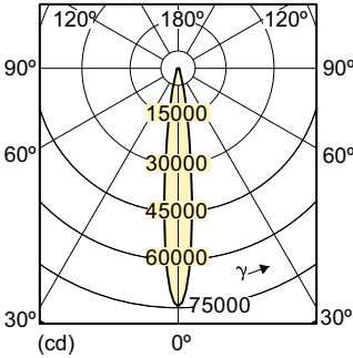
Light Distribution Diagram - MC CDM-R Elite 70W/930 E26 PAR30L 10D
