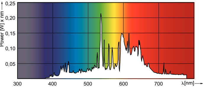
Spectral Power Distribution Colour - MC CDM-R Elite 70W/930 E26 PAR30L 10D
