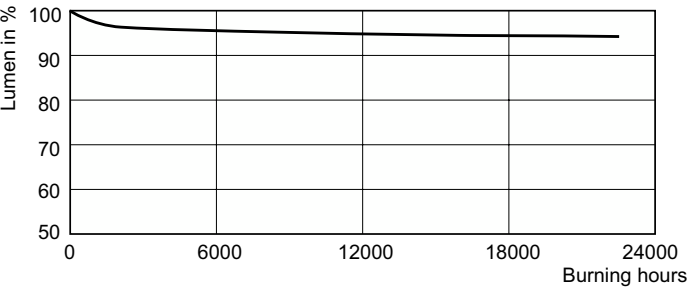
Lumen Maintenance Diagram - SOX E 131W BY22d T65 1SL/6
