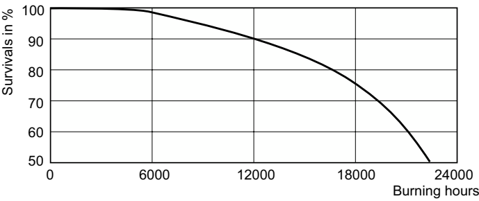
Life Expectancy Diagram - SOX E 131W BY22d T65 1SL/6
