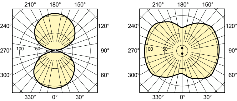
Light Distribution Diagram - SOX E 131W BY22d T65 1SL/6
