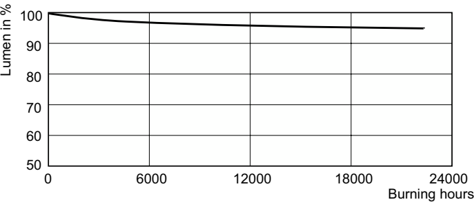
Lumen Maintenance Diagram - SOX 35W BY22d T50 1SL/12
