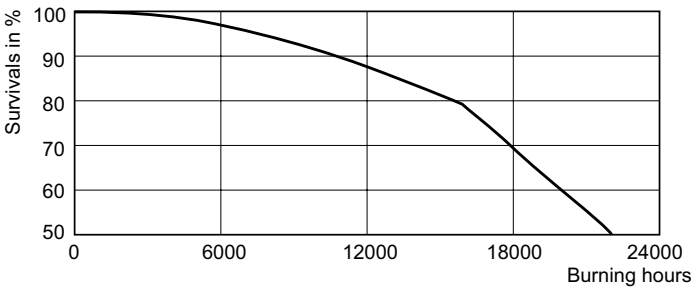
Life Expectancy Diagram - SOX 35W BY22d T50 1SL/12
