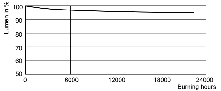
Lumen Maintenance Diagram - SOX 55W BY22d 1SL/12
