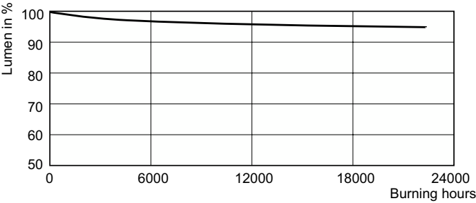
Lumen Maintenance Diagram - SOX 135W BY22d T65 1SL/12
