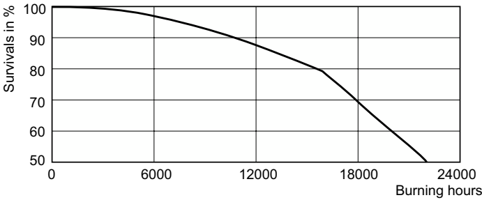
Life Expectancy Diagram - SOX 135W BY22d T65 1SL/12
