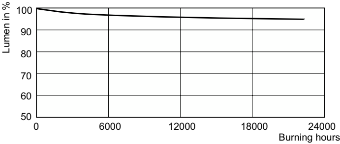
Life Expectancy Diagram - SOX 180W BY22d 1SL/6 Lumen Maintenance Diagram - SOX 180W BY22d 1SL/6
