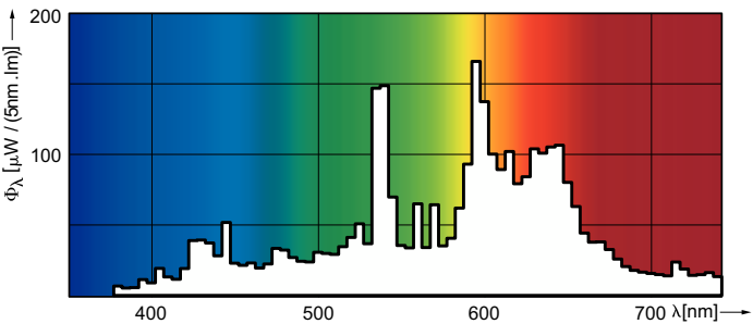
Spectral Power Distribution Colour - MASTERColor CDM-T Elite 100W/930.1CT/12
