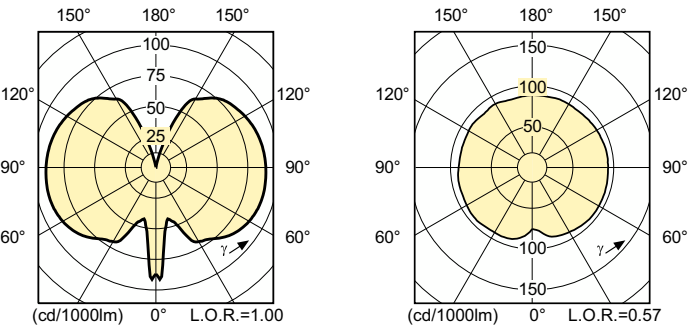
Light Distribution Diagram - MASTERColor CDM-T Elite 100W/930.1CT/12
