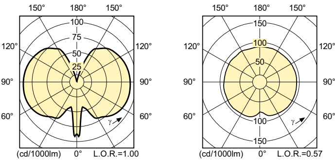
Light Distribution Diagram - MASTERColor CDM-T Elite 100W/930.1CT/12
