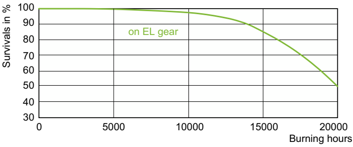
Life Expectancy Diagram - MASTER CDM-T Elite 100W/930 G12 1CT/12
