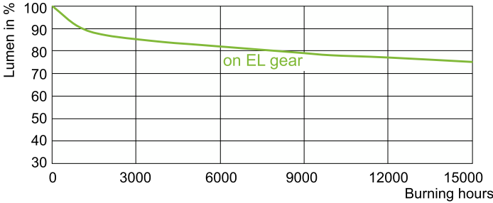
Lumen Maintenance Diagram - MC CDM-T Elite 20W830 G12 T6 CL 1CT/12
