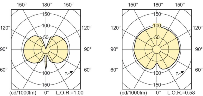
Light Distribution Diagram - MASTERC CDM-TC Elite 20W/830 G8.5 ICT/12
