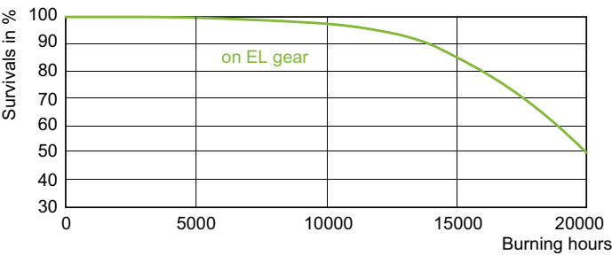
Life Expectancy Diagram - MASTERC CDM-TC Elite 70W/930 G8.5 OEM
