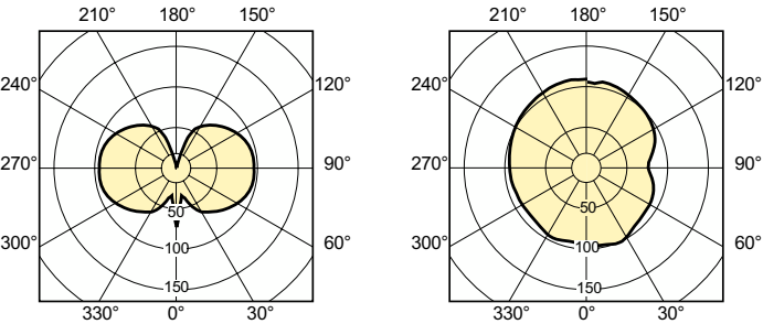
Light Distribution Diagram - MASTERC CDM-TC Elite 70W/930 G8.5 OEM
