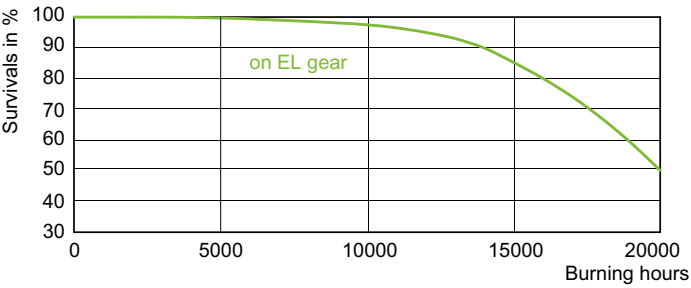
Life Expectancy Diagram - MasterColor CDM-TC 50W/930 G8.5
