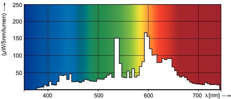
Spectral Power Distribution Colour - MasterColor CDM-TC 50W/930 G8.5
