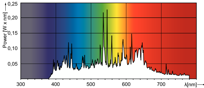
Spectral Power Distribution Colour - MASTERC CDM-T Elite 70W/942 G12
