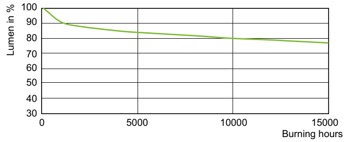
Lumen Maintenance Diagram - MASTERC CDM-T Elite 70W/942 G12
