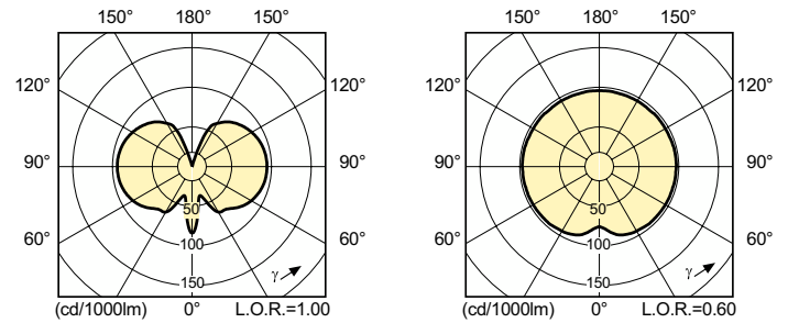
Light Distribution Diagram - MASTERC CDM-T Elite 70W/942 G12
