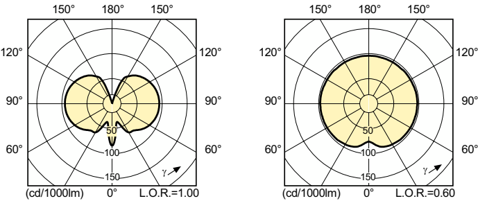
Light Distribution Diagram - MASTERC CDM-T Elite 70W/942 G12 1CT/12
