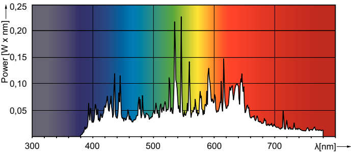
Spectral Power Distribution Colour - MASTERC CDM-T Elite 70W/942 G12 1CT/12
