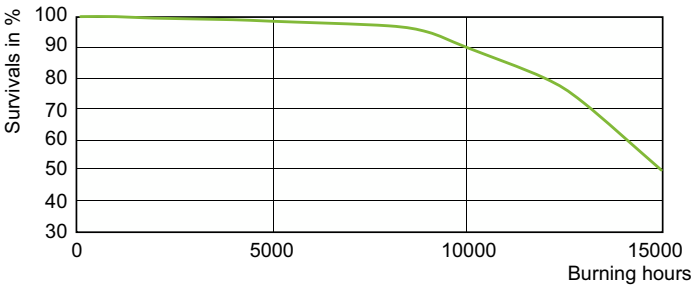
Life Expectancy Diagram - MASTERC CDM-T Elite 70W/942 G12 1CT/12
