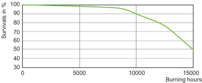
Life Expectancy Diagram - MASTERC CDM-TC Elite 70W/942 G8.5 OEM
