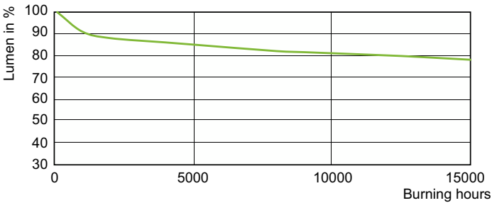
Lumen Maintenance Diagram - MASTERC CDM-TC Elite 70W/942 G8.5 OEM
