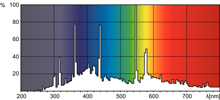
Spectral Power Distribution Colour - MSD Platinum 14 R UNP/24
