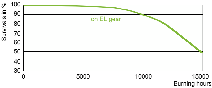
Life Expectancy Diagram - MASTERColour CDM-T Fresh 70W/740 G12 1CT
