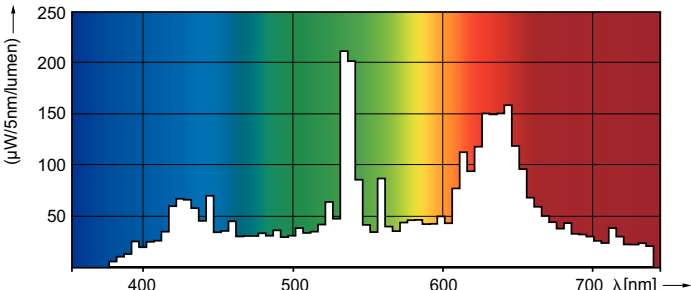
Spectral Power Distribution Colour - MASTERColour CDM-T Fresh 70W/740 G12 1CT
