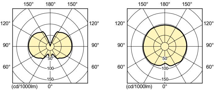
Light Distribution Diagram - MASTERColour CDM-T Fresh 70W/740 G12 1CT
