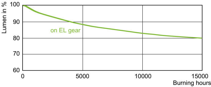
Lumen Maintenance Diagram - MASTERColour CDM-T Fresh 70W/740 G12 1CT
