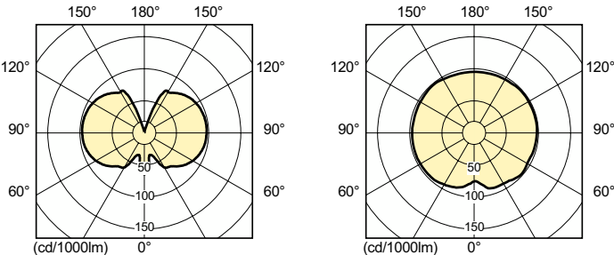
Light Distribution Diagram - MASTERColour CDM-T Fresh 70W/740 G12 1CT
