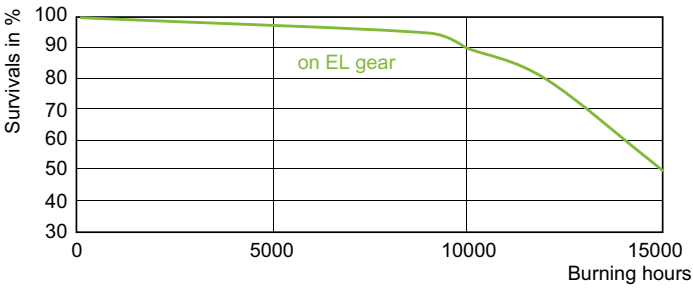
Life Expectancy Diagram - MASTERColour CDM-TC Fresh 70W/740 G8.5
