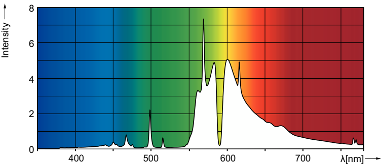
Spectral Power Distribution Colour - HPS AGRO Plus 1000W DE EL
