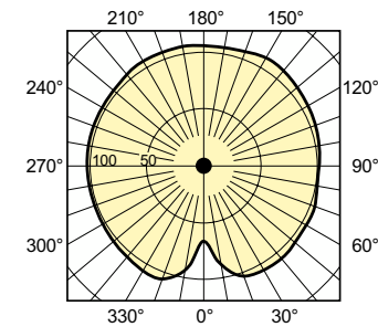
Light Distribution Diagram - MST SON-T APIA Plus Hg Free 100W E40 1SL
