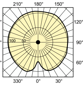
Light Distribution Diagram - MST SON-T APIA Plus Hg Free 250W E40 1SL
