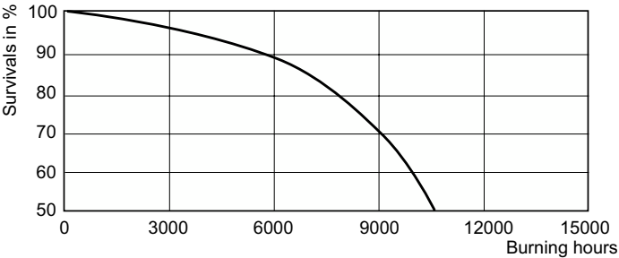
Life Expectancy Diagram - MHN-TD Essential 150W/730 Rx7s 1CT/12
