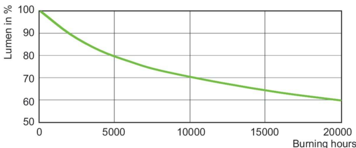
Lumen Maintenance Diagram - HPI-T Plus 400W/645 E40 1SL/12
