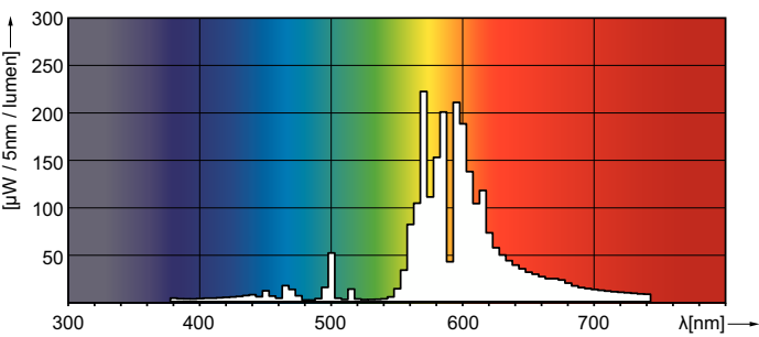
Spectral Power Distribution Colour - MST SON-T PIA Plus 100W E40 1SL/12
