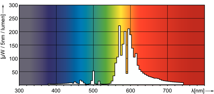
Spectral Power Distribution Colour - MST SON-T PIA Plus 150W E40 1SL/12
