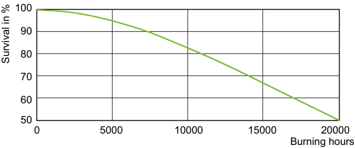
Life Expectancy Diagram - MASTER HPI-T Plus 250W/643 E39 1SL
