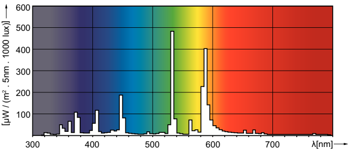
Spectral Power Distribution Colour - MASTER HPI-T Plus 250W/643 E39 1SL
