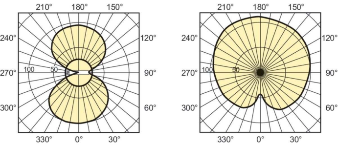
Light Distribution Diagram - MASTER HPI-T Plus 250W/643 E39 1SL
