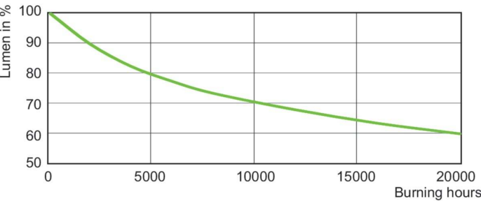
Lumen Maintenance Diagram - MASTER HPI-T Plus 250W/643 E39 1SL
