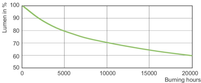
Lumen Maintenance Diagram - MASTER HPI-T Plus 400W/643 E39 1SL
