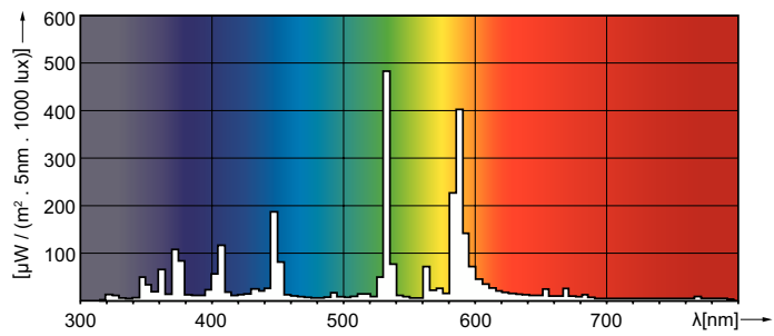
Spectral Power Distribution Colour - MASTER HPI-T Plus 400W/643 E39 1SL
