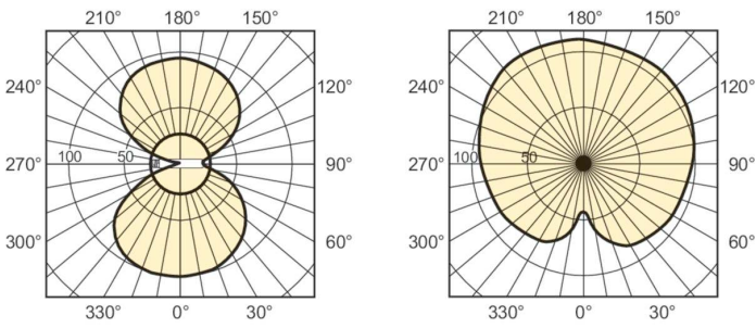
Light Distribution Diagram - MASTER HPI-T Plus 400W/643 E39 1SL
