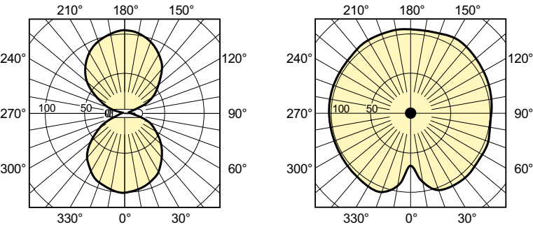
Light Distribution Diagram - MASTER SON-T PIA Eco 220W E E40 1SL/12
