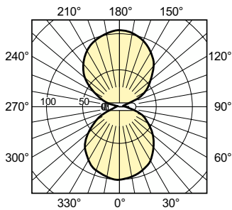
Light Distribution Diagram - SON-T 150W E E40 1SL
