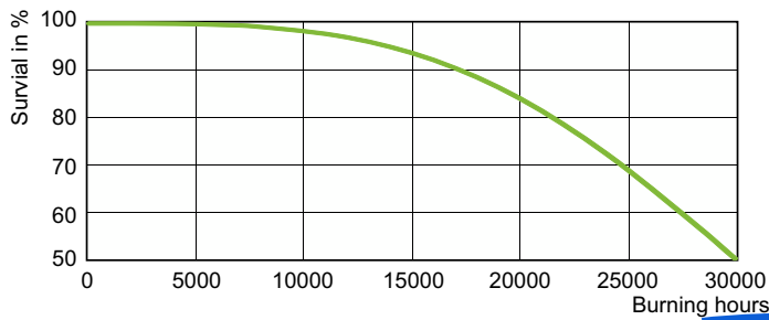
Life Expectancy Diagram - SON-T 150W E E40 1SL
