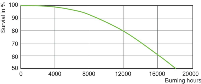
Life Expectancy Diagram - MASTER CityWh CDO-TT Plus 250W/940 E40
