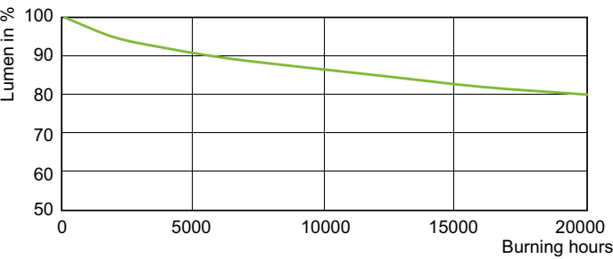
Lumen Maintenance Diagram - MASTER CityWh CDO-TT Plus 250W/940 E40
