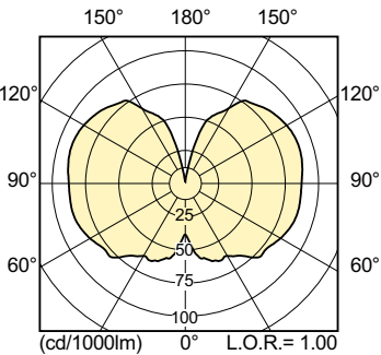
Light Distribution Diagram - MASTER CityWh CDO-TT Plus 250W/940 E40
