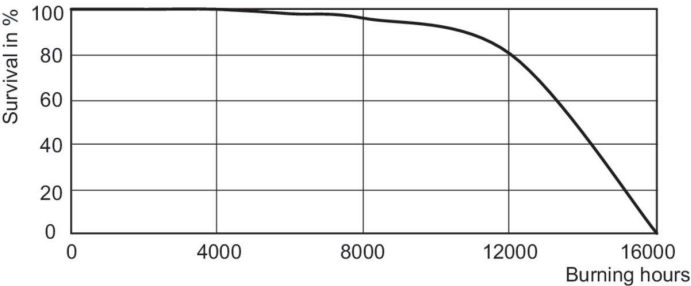
Life Expectancy Diagram - CDM70/PAR38/SP/3K ALTO ELITE 12PK
