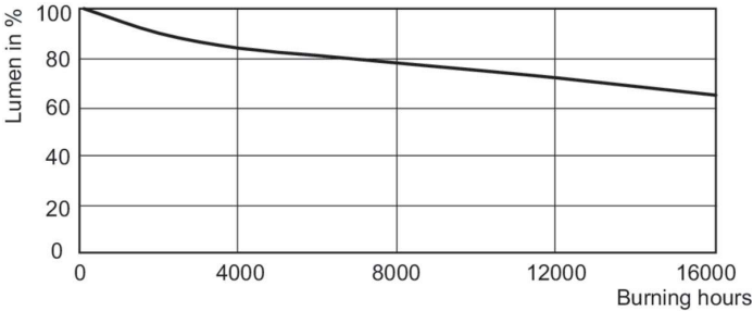
Lumen Maintenance Diagram - CDM70/PAR38/FL/3K ALTO ELITE 12PK
