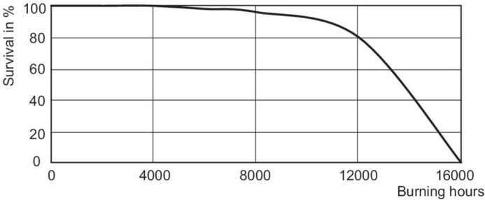
Life Expectancy Diagram - CDM70/PAR38/FL/3K ALTO ELITE 12PK
