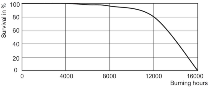
Life Expectancy Diagram - CDM100/PAR38/SP/3K ALTO ELITE 12PK
