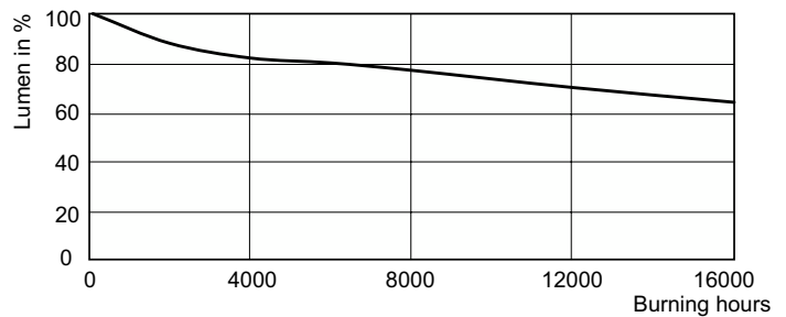
Lumen Maintenance Diagram - CDM100/PAR38/FL/4K ALTO ELITE 12PK
