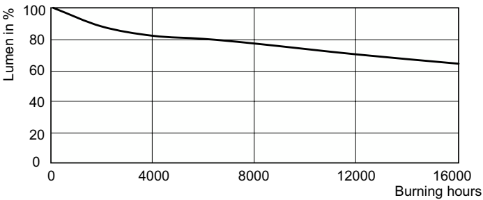
Lumen Maintenance Diagram - CDM100/PAR38/FL/4K ALTO ELITE 12PK
