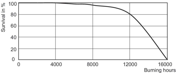
Life Expectancy Diagram - CDM100/PAR38/FL/4K ALTO ELITE 12PK
