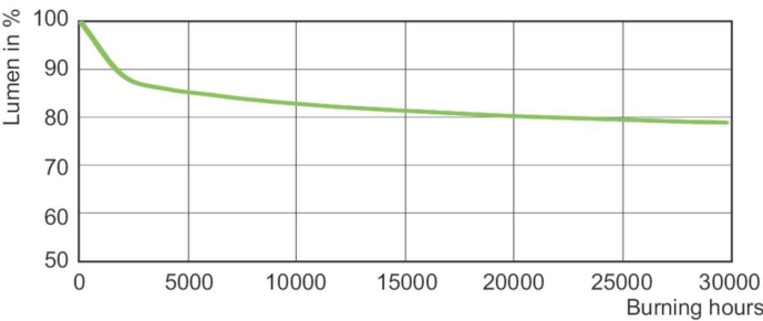
Lumen Maintenance Diagram - SON-T 70W E E27 1CT/12
