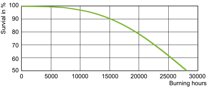
Life Expectancy Diagram - SON-T 70W E E27 1CT/12
