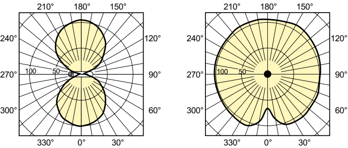
Light Distribution Diagram - SON-T 70W E E27 1CT/12
