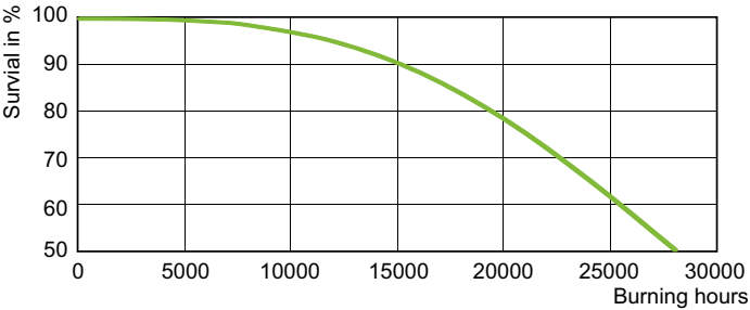
Life Expectancy Diagram - SON-T 70W E E27 1CT/12
