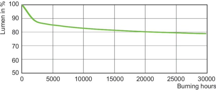
Lumen Maintenance Diagram - SON-T 70W E E27 1CT/12
