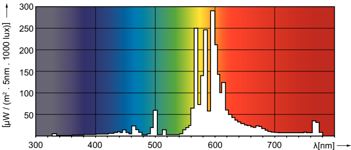
Spectral Power Distribution Colour - SON-T 70W E E27 1CT/12
