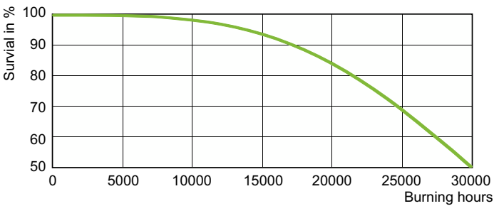
Life Expectancy Diagram - SON-T 100W E E40 1SL/12
