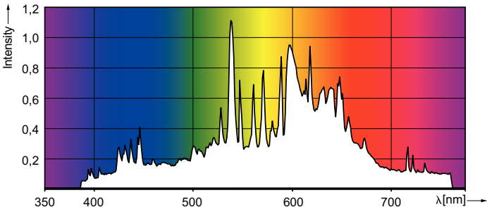
Spectral Power Distribution Colour - MASTERC CDM-TMW Elite 315W/930 1CT/12
