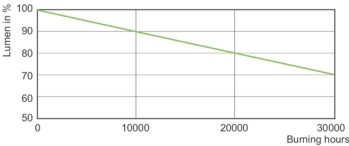
Lumen Maintenance Diagram - MASTERC CDM-TMW Elite 315W/930 1CT/12
