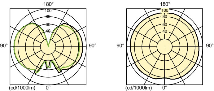
Light Distribution Diagram - MASTERC CDM-TMW Elite 315W/930 1CT/12
