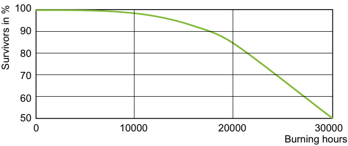
Life Expectancy Diagram - MASTERC CDM-TMW Elite 315W/930 1CT/12
