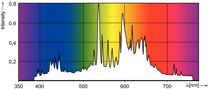
Spectral Power Distribution Colour - CDM T9 ELITE 210W/930/U/E NA
