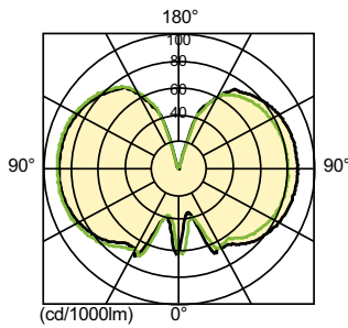
Light Distribution Diagram - CDM-T Elite 315W/942 PGZ18.1CT/12
