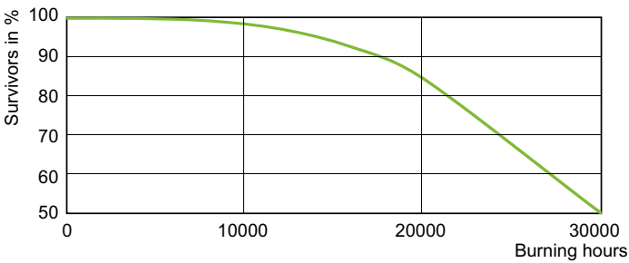
Life Expectancy Diagram - MASTERC CDM-TM Elite 315W/942 1CT/12
