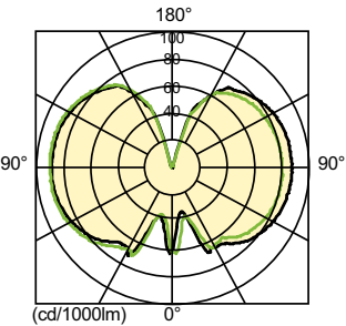
Light Distribution Diagram - MASTERC CDM-TMW Elite 315W/942 1CT/12
