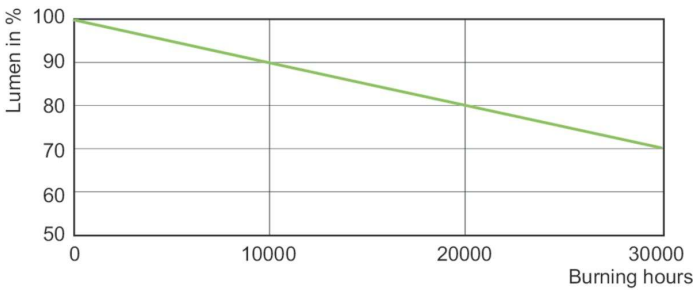
Lumen Maintenance Diagram - MASTERC CDM-TM Elite 315W/942 1CT/12
