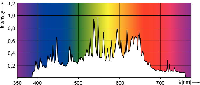
Spectral Power Distribution Colour - MASTERC CDM-TMW Elite 315W/942 1CT/12
