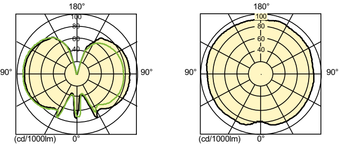
Light Distribution Diagram - MASTERC CDM-TMW Elite 210W/942 1CT/12
