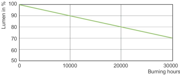
Lumen Maintenance Diagram - MASTERC CDM-TM Elite 210W/942 1CT/12
