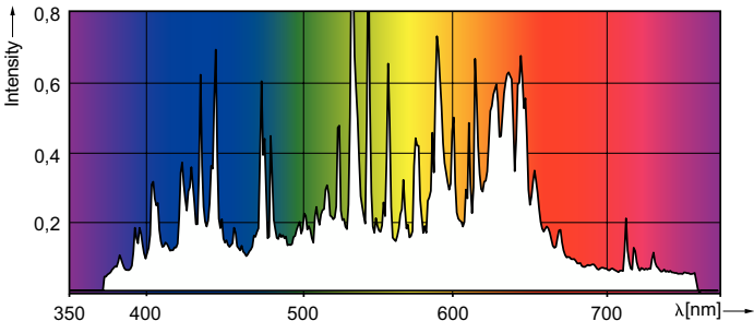
Spectral Power Distribution Colour - MASTERC CDM-TMW Elite 210W/942 1CT/12
